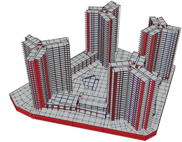
AllSancak Residences High-Rise Concrete Building Total Area: 110.000 sq. meters
