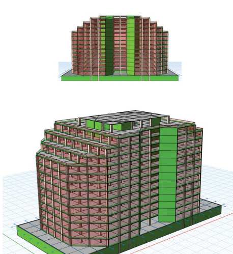
Hexagon Ankara High-Rise Concrete Building Number of Floors: 13-storey
