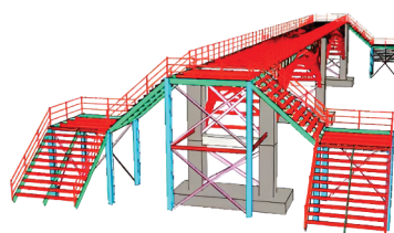
Santo Domingo Pedestrian Bridge Steel Structure Main Span: 54 meters
